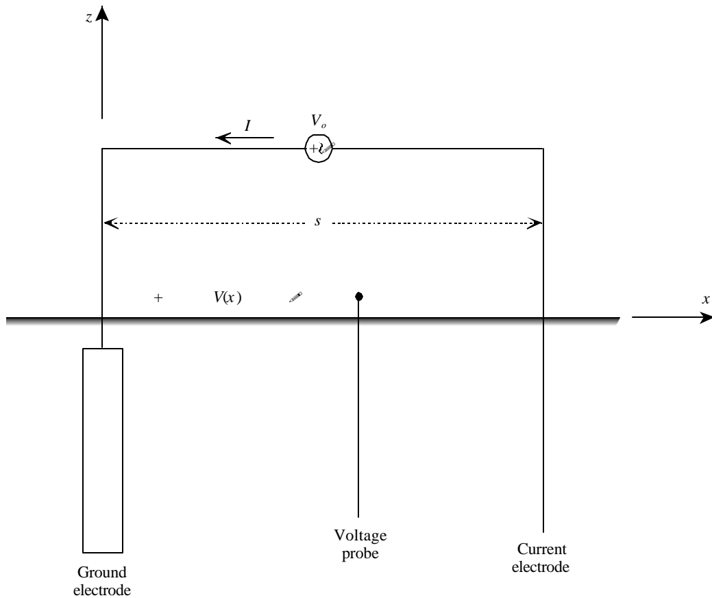
Figure 2. Fall-in-potential method.
